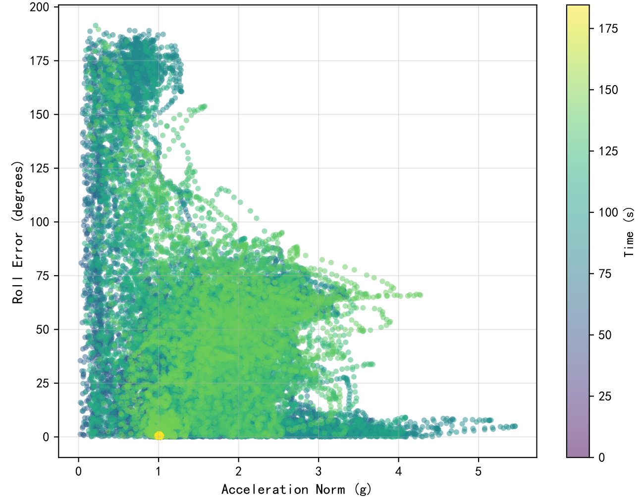
Raw Accelerometer (No Filtering)
